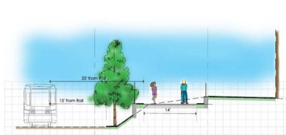
ALTERNATIVE W9B CROSS SECTION: DOUBLE KNEE-WALL
