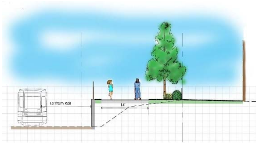
ALTERNATIVE W9B CROSS SECTION: SINGLE WALL
