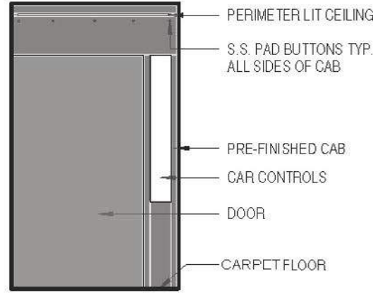
HIGH SCHOOL 'ELEVATOR 1' EAST ELEVATION
