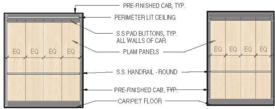
MIDDLE SCHOOL 'ELEVATOR 2' NORTH ELEVATION
