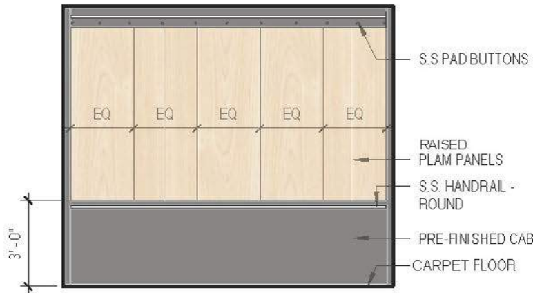
HIGH SCHOOL 'ELEVATOR 1' NORTH ELEVATION
