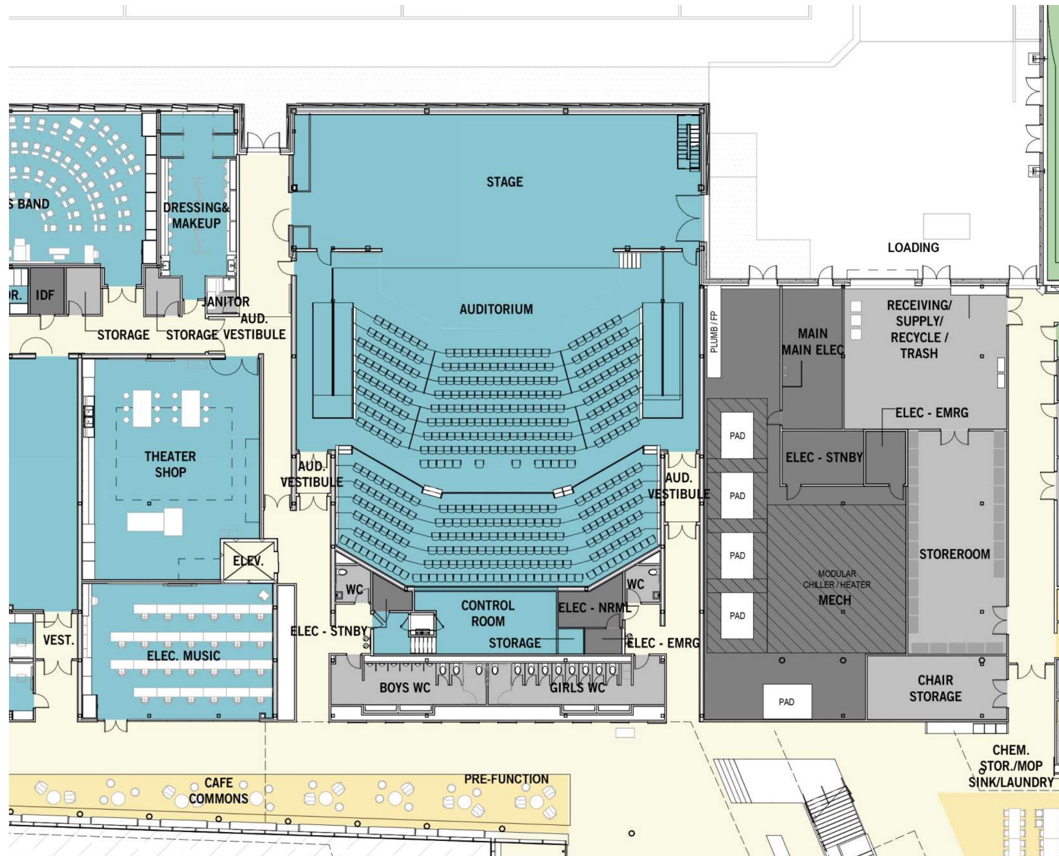
AUDITORIUM LEVEL 01
