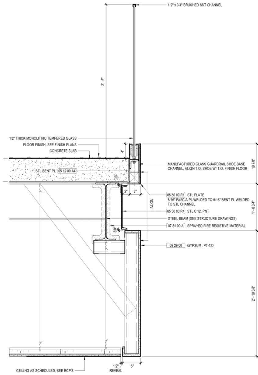
CURRENT RAIL DETAIL
