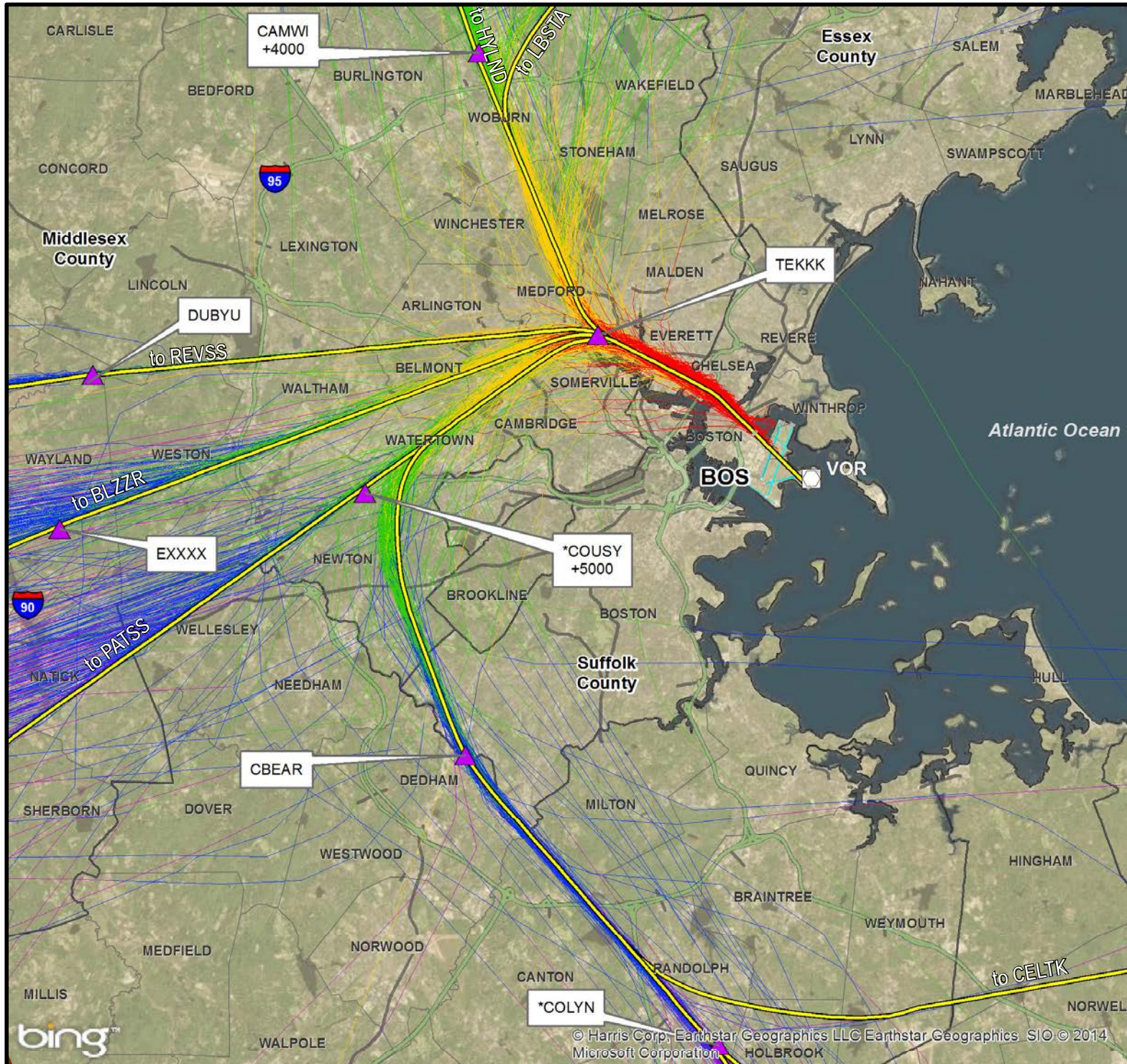
Figure 4 Runway 33L RNAV Flight Tracks with Altitudes
