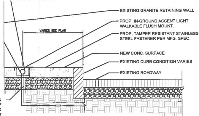
IN GROUND UP-LIGHT TYPE (U)
