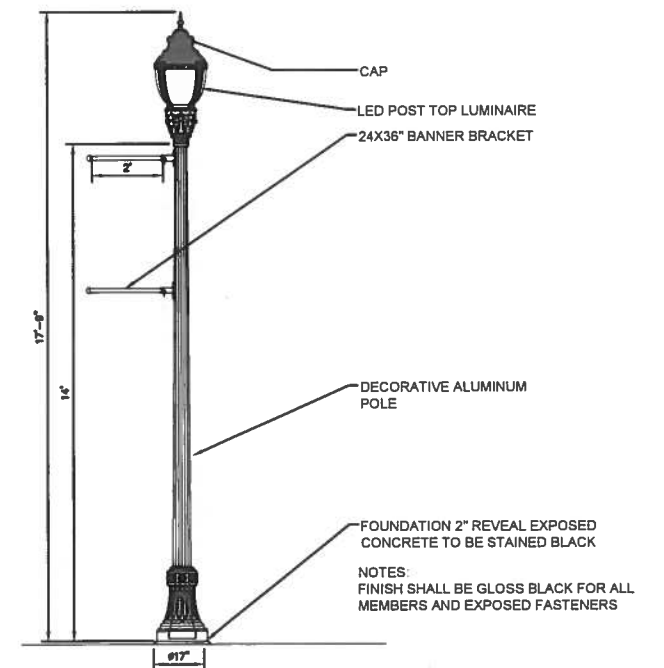
LIGHTPOLE AND LUMINAIRE TYPE (C) POSTTOP
