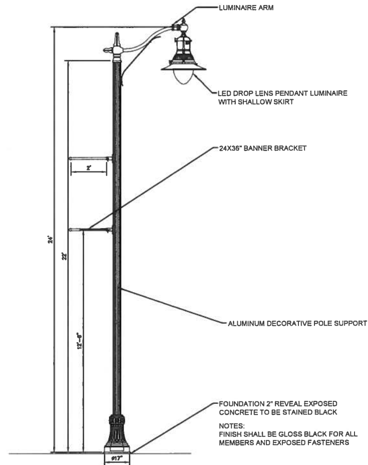
LIGHTPOLE AND LUMINAIRE TYPE (A) SINGLE
