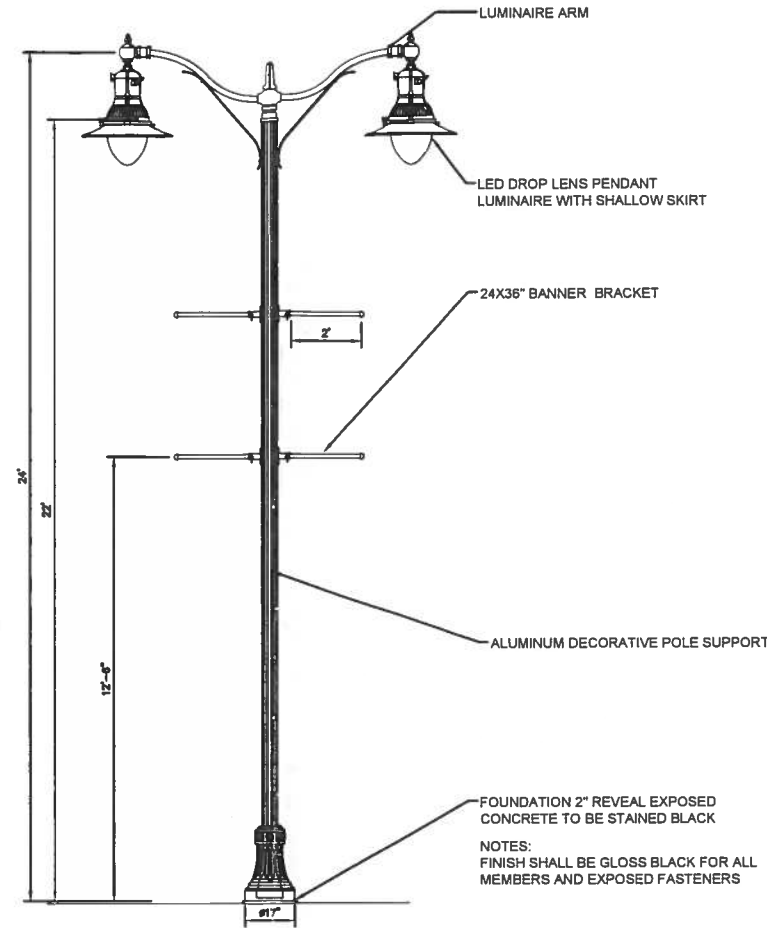
LIGHTPOLE AND LUMINAIRE TYPE (B) DOUBLE
