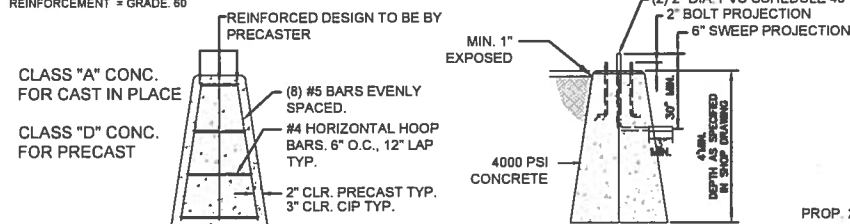
CEMENT CONCRETE LIGHT POLE FOUNDATION
