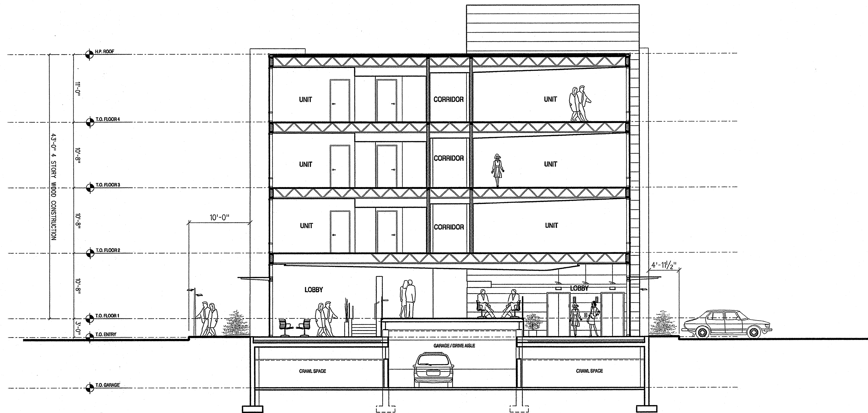
1 TYPICAL CROSS SECTION (AT LOBBY) SCALE: 1" = 8'
