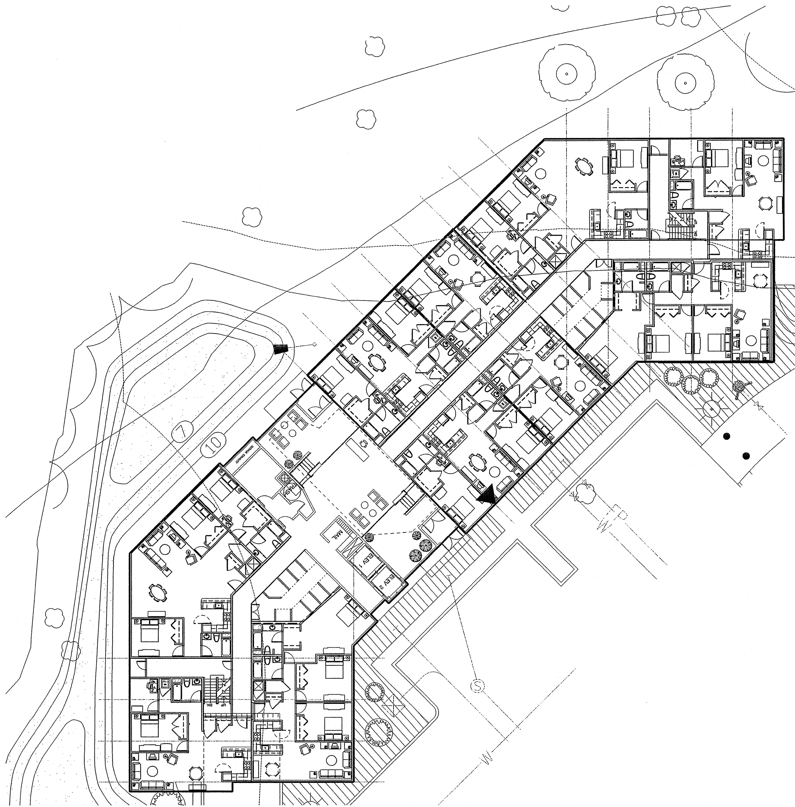
2 BUILDING PLAN BUILDING D - TYPICAL FLOOR SCALE: 1" = 16'
