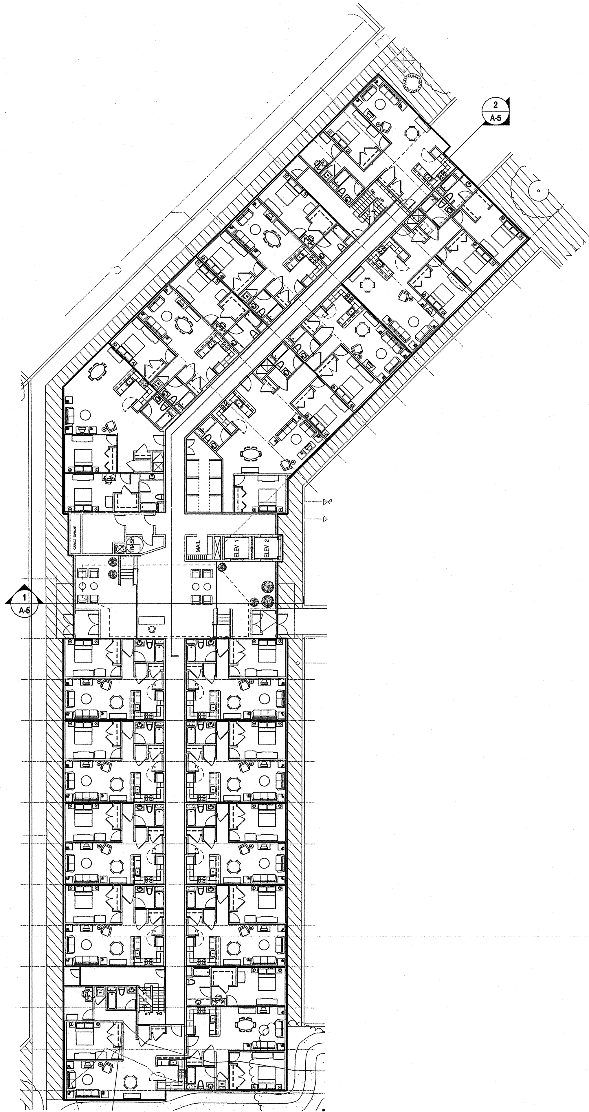
1 BUILDING PLAN SCALE: 1" = 16'
