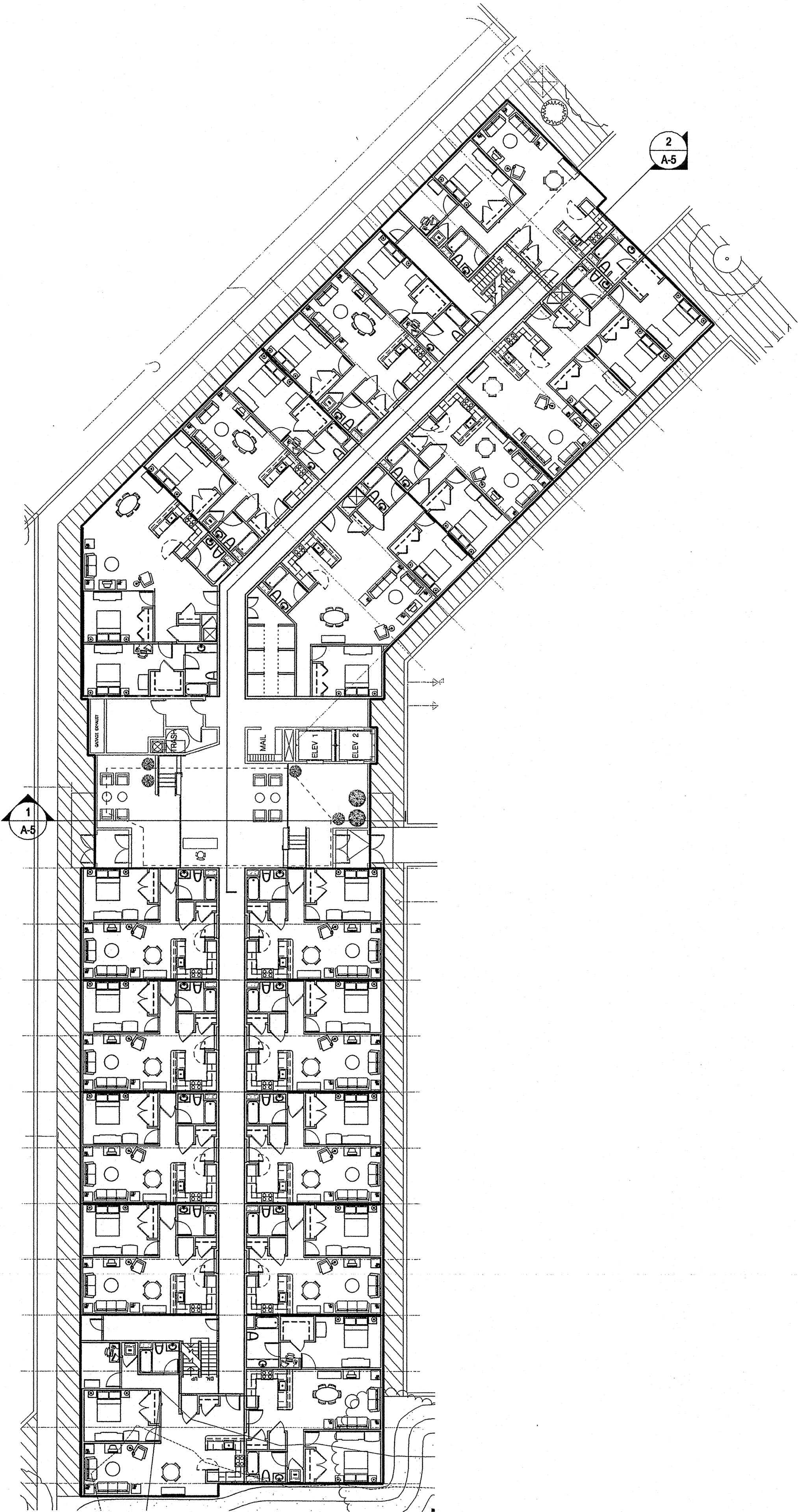
2 BUILDING PLAN SCALE: 1" = 16'
