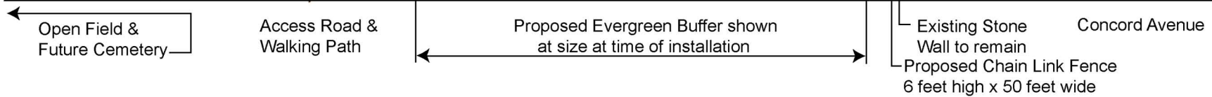
ELEVATION VIEW OF PROPOSED COMPOUND LOOKING WEST
